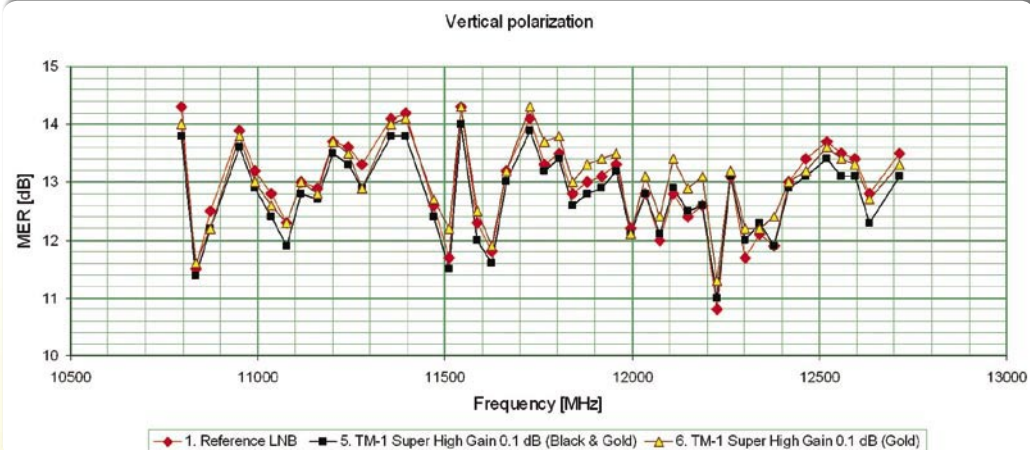
■ Fig. 5. Noise performance of the 0.1 dB models – vertical polarization.
