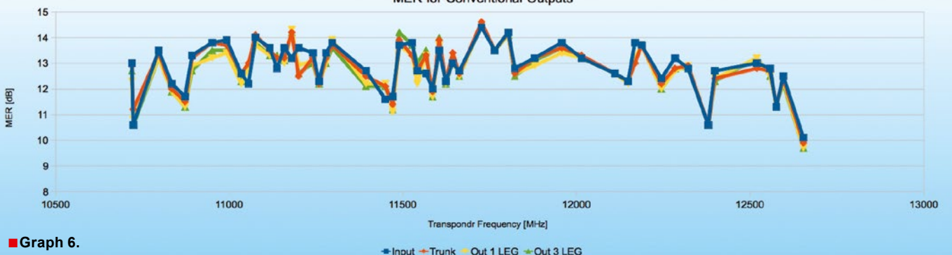
SUS 5581/33 NFA LEGACY MER for Conventional Outputs
