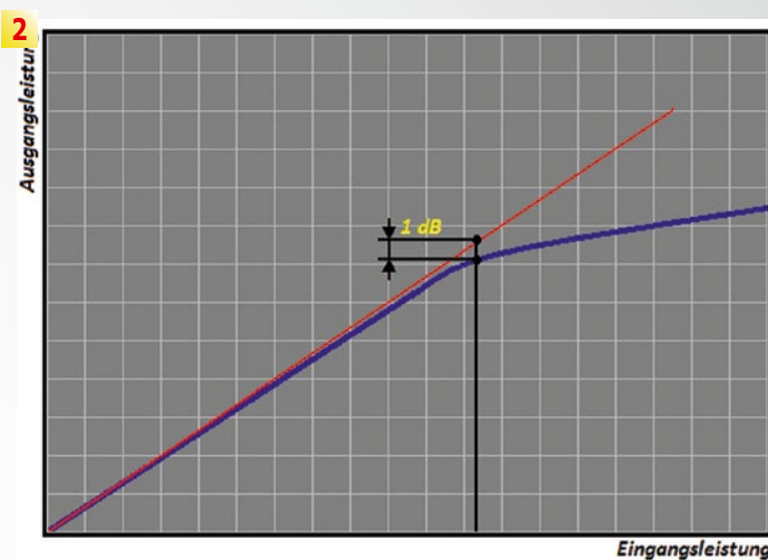
1: Intermodulation occurs directly next to the wanted signal - see the red labeled signals
