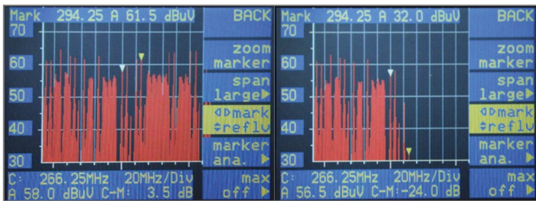
■ Example with a UHF filter of a pay TV operator: The left picture shows the whole CATV spectrum without any filter. The right picture shows the result of using a low pass filter with a cut-off frequency of 296 MHz.
