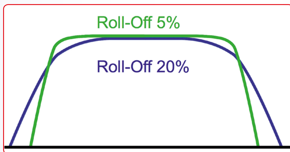
■ Figure 1. With smaller roll-offs, transponders can be squeezed closer to one another.
